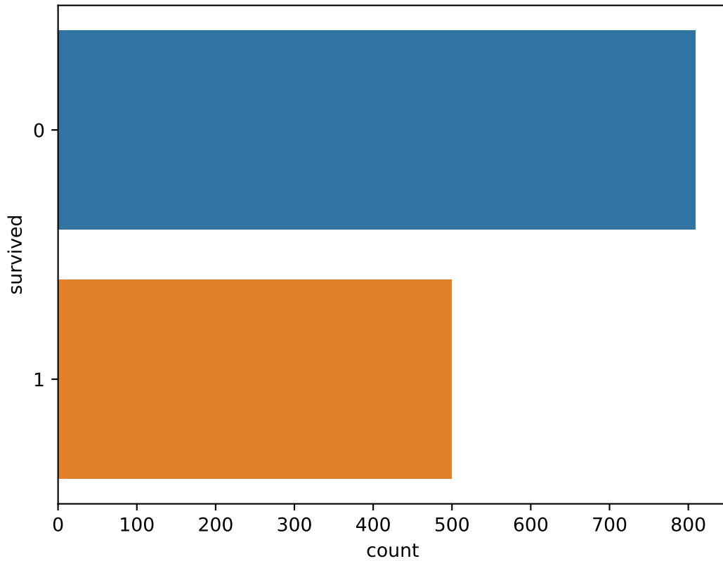
Target distribution
